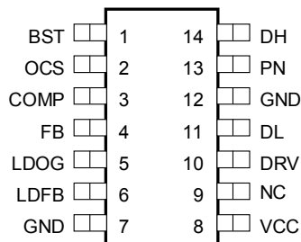
SOIC-14 TOP VIEW
