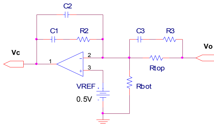
Fig. 5. Compensation network
