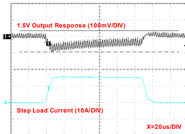
Transient Response
