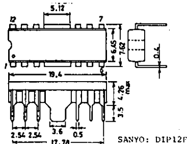
Package Dimensions 3022A (unit: mm)
