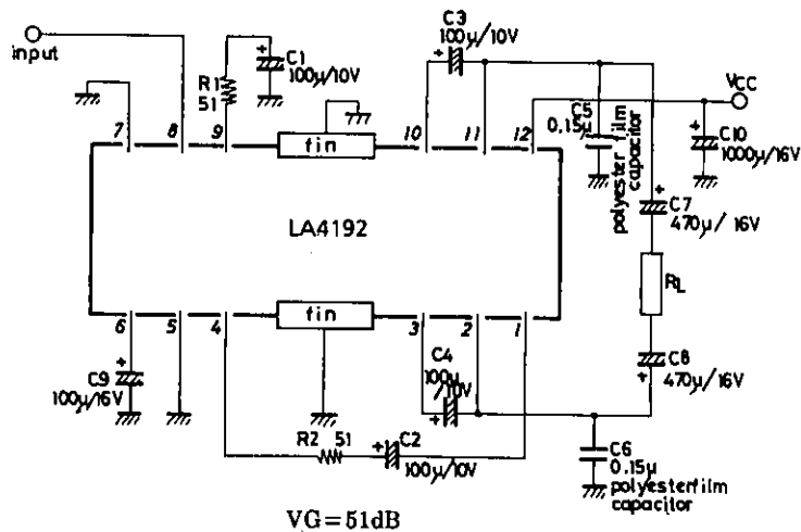
Sample application circuit 2: Bridge amp. connected
