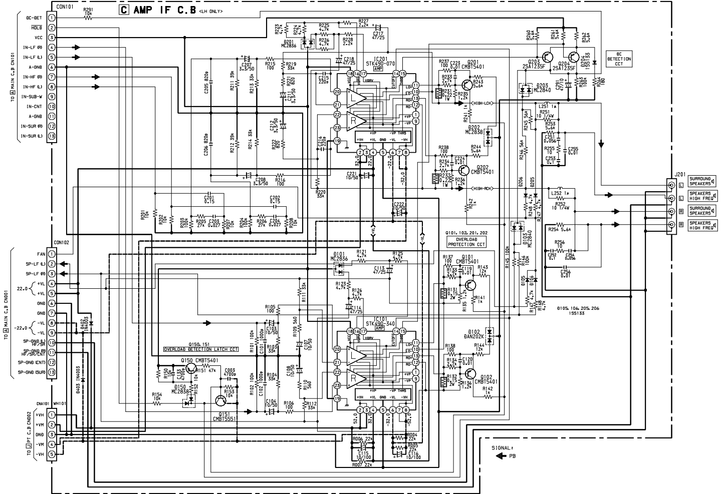
SCHEMATIC DIAGRAM - 7 (LH : AMP IF)
