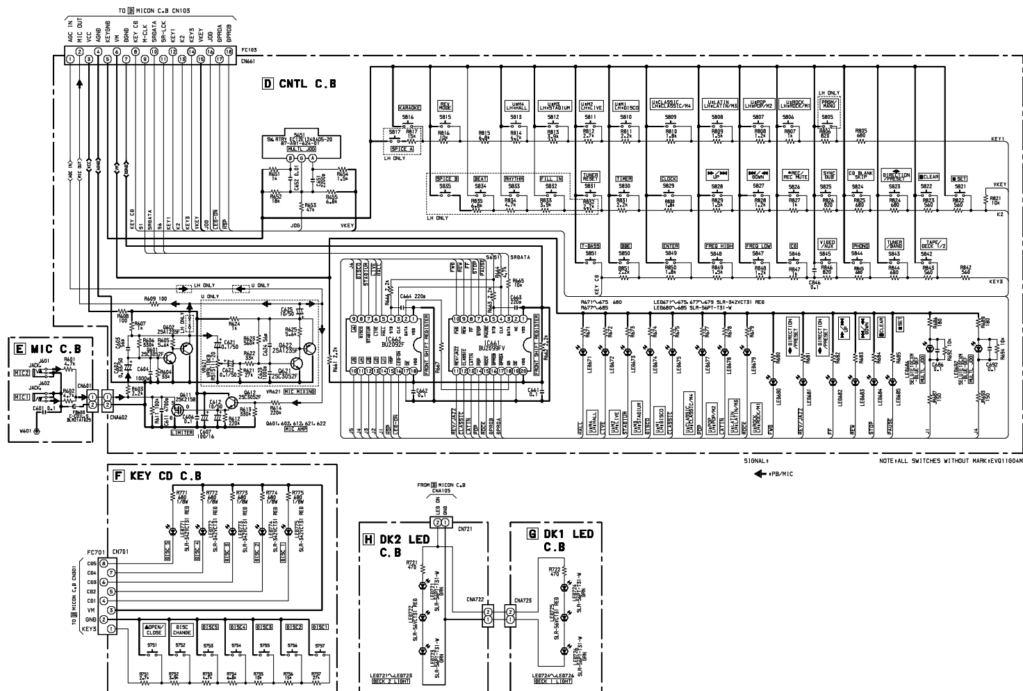
SCHEMATIC DIAGRAM - 5 (CNTL / MIC / KEY CD / DK1 LED / DK2 LED)
