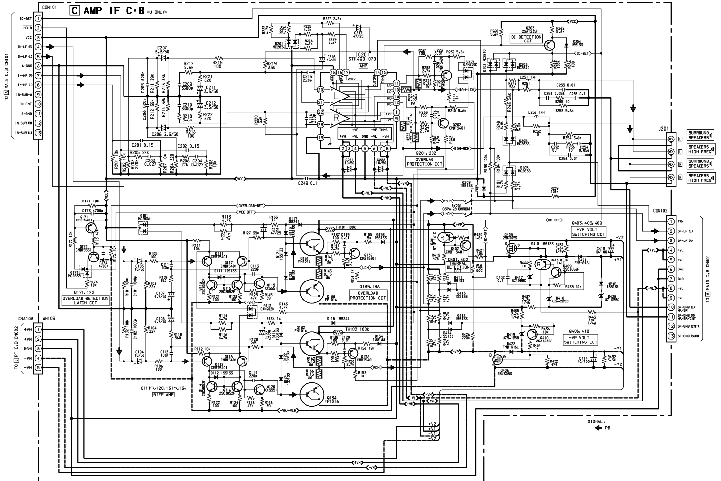
SCHEMATIC DIAGRAM - 6 (U : AMP IF)
