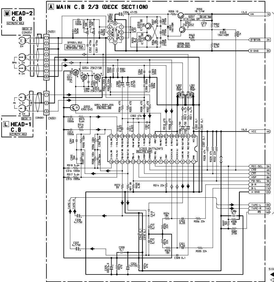
SCHEMATIC DIAGRAM - 2 (MAIN 2 / 3 <DECK> / HEAD - 1 / HEAD - 2 )
