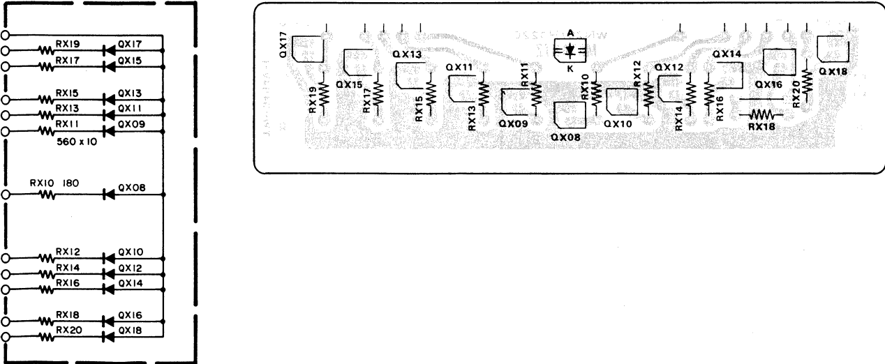
11.8 LED Level Meter Assembly (PX02) Schematic Diagram and Component Locations
