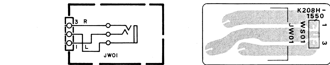
11.5 Head Phone Assembly (PW00) Schematic Diagram and Component Locations
