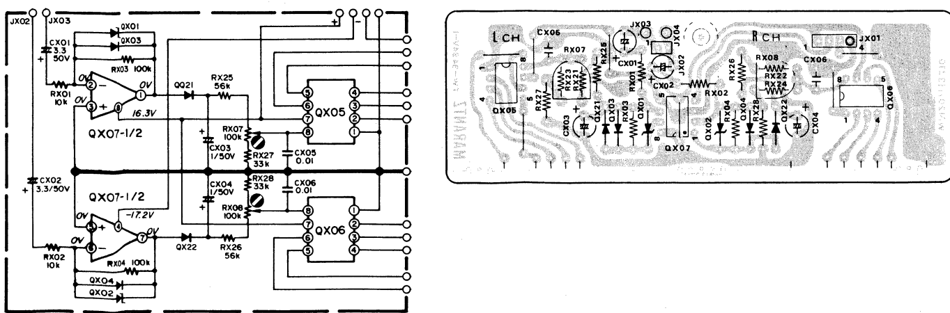
11.6 Tone Control Assembly (PE00) Schematic Diagram and Component Locations
