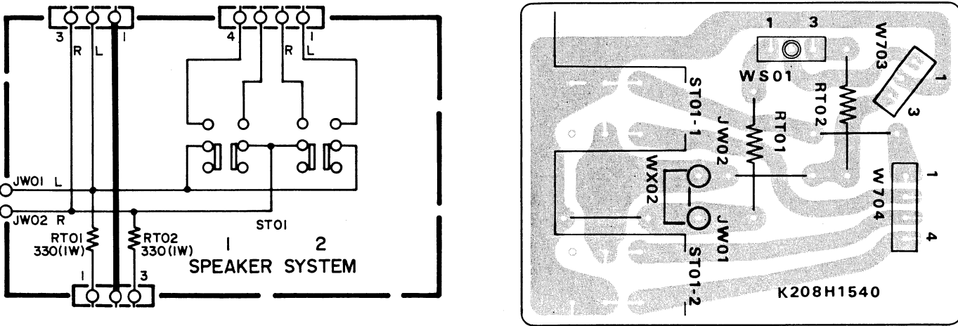
11.4 SP. Switch Assembly (PT00) Schematic Diagram and Component Locations
