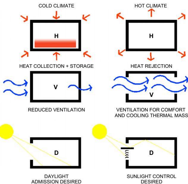
Fig. 5. Some building design strategies for cold and hot climates. Source: [144].
