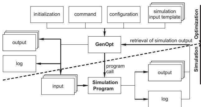
Fig. 2. Interface between GenOpt and a simulation program. Source: [18].
