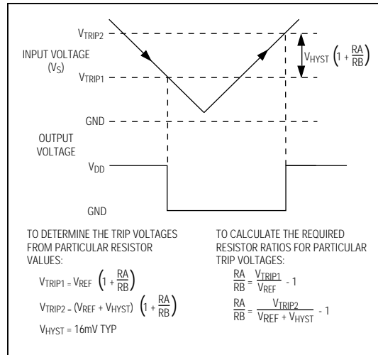
Figure 3. Undervoltage/Overvoltage Detector Waveforms and Formulas
