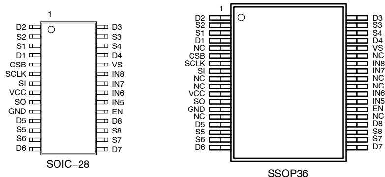
Figure 3. Pin Connections
