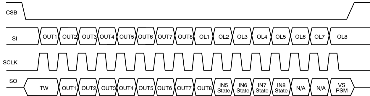
Figure 23. SPI Frame
