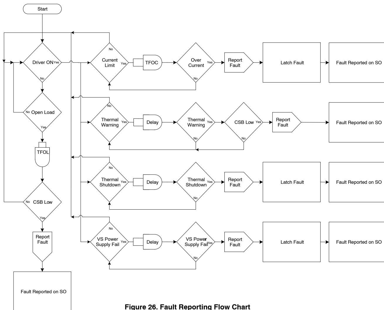
Figure 26. Fault Reporting Flow Chart
