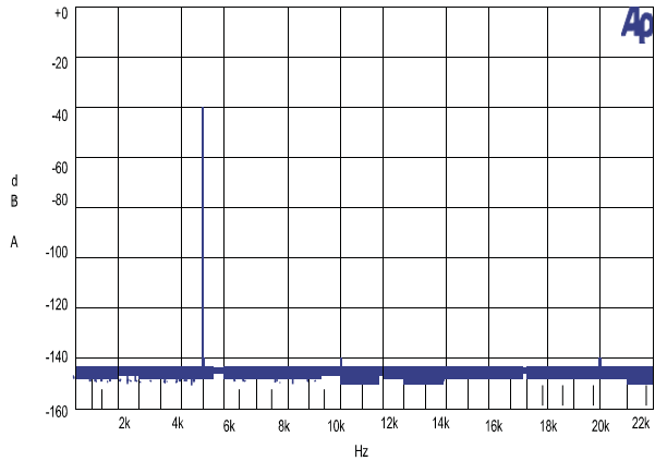
FFT Analysis. f = 5\text{kHz} . P_o = 100\text{mW} 4Ω loading. THD = -101dB (0.0009%)
