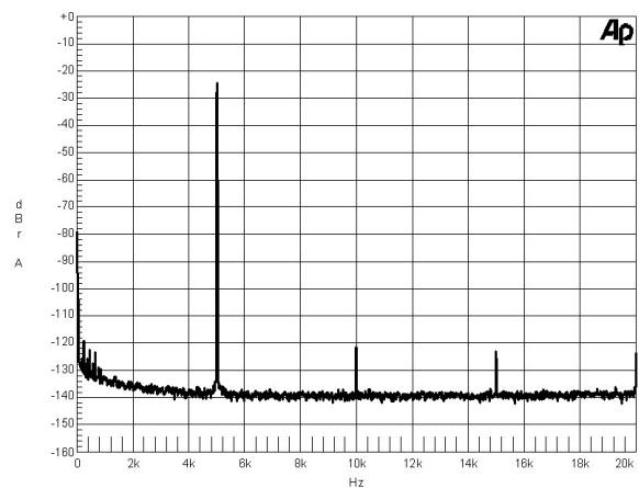
f = 5\text{kHz} . P_o = 1\text{W} . 4Ω loading. THD = 0.002%.
