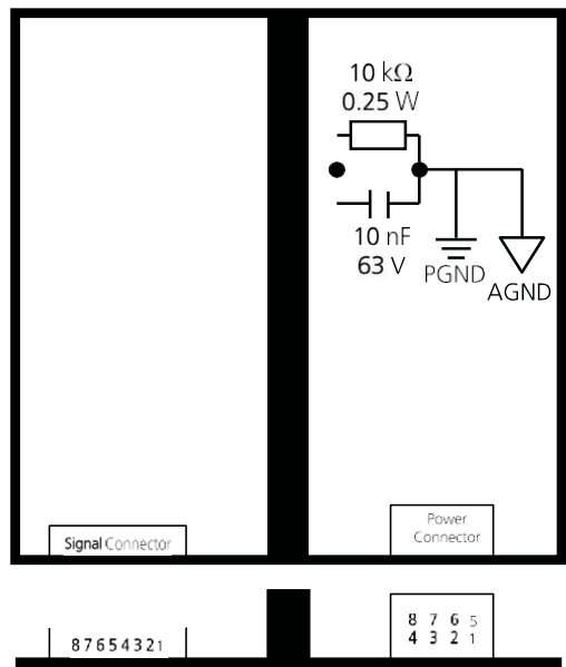
Figure 3: ICEpower250A-IC connectors.
