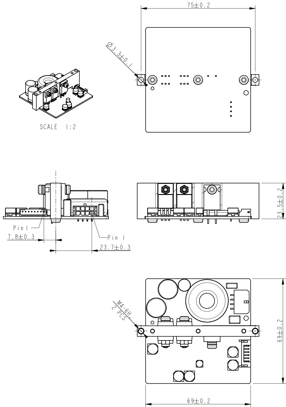
Figure 17: Physical dimensions ICEpower250A-IC.
