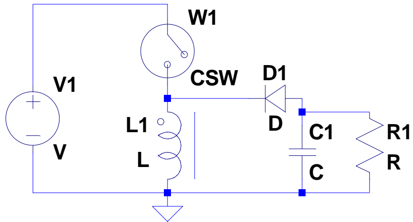
1) Inverting boost-buck
