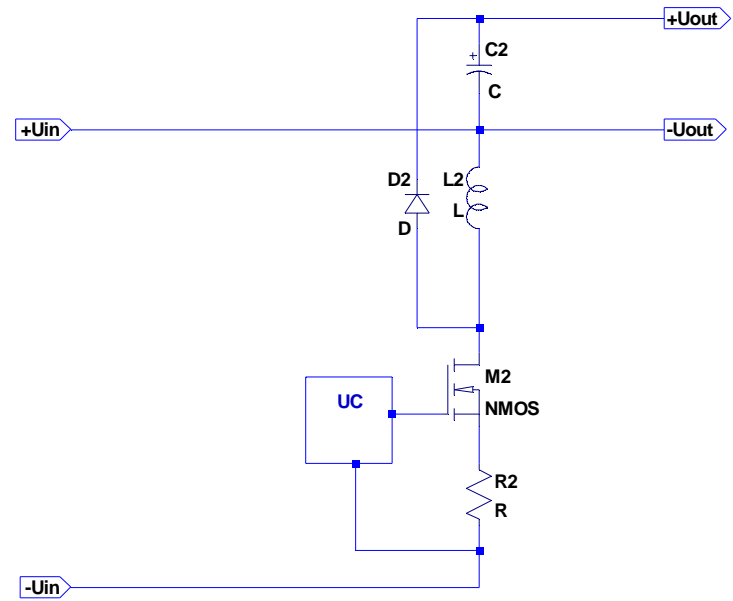
Inverting buck-boost
