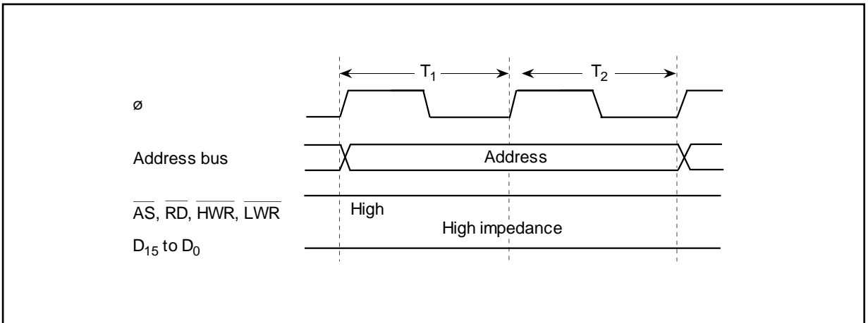
Pin States During On-Chip Memory Access
