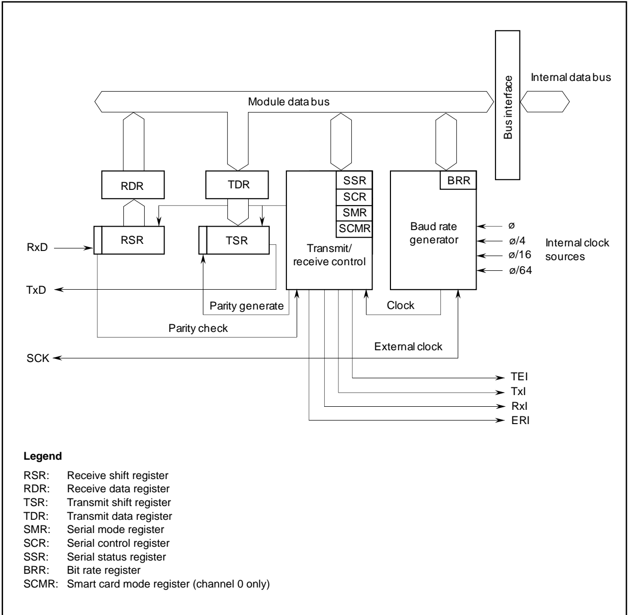
Serial Communication Interface Block Diagram (One Channel)
