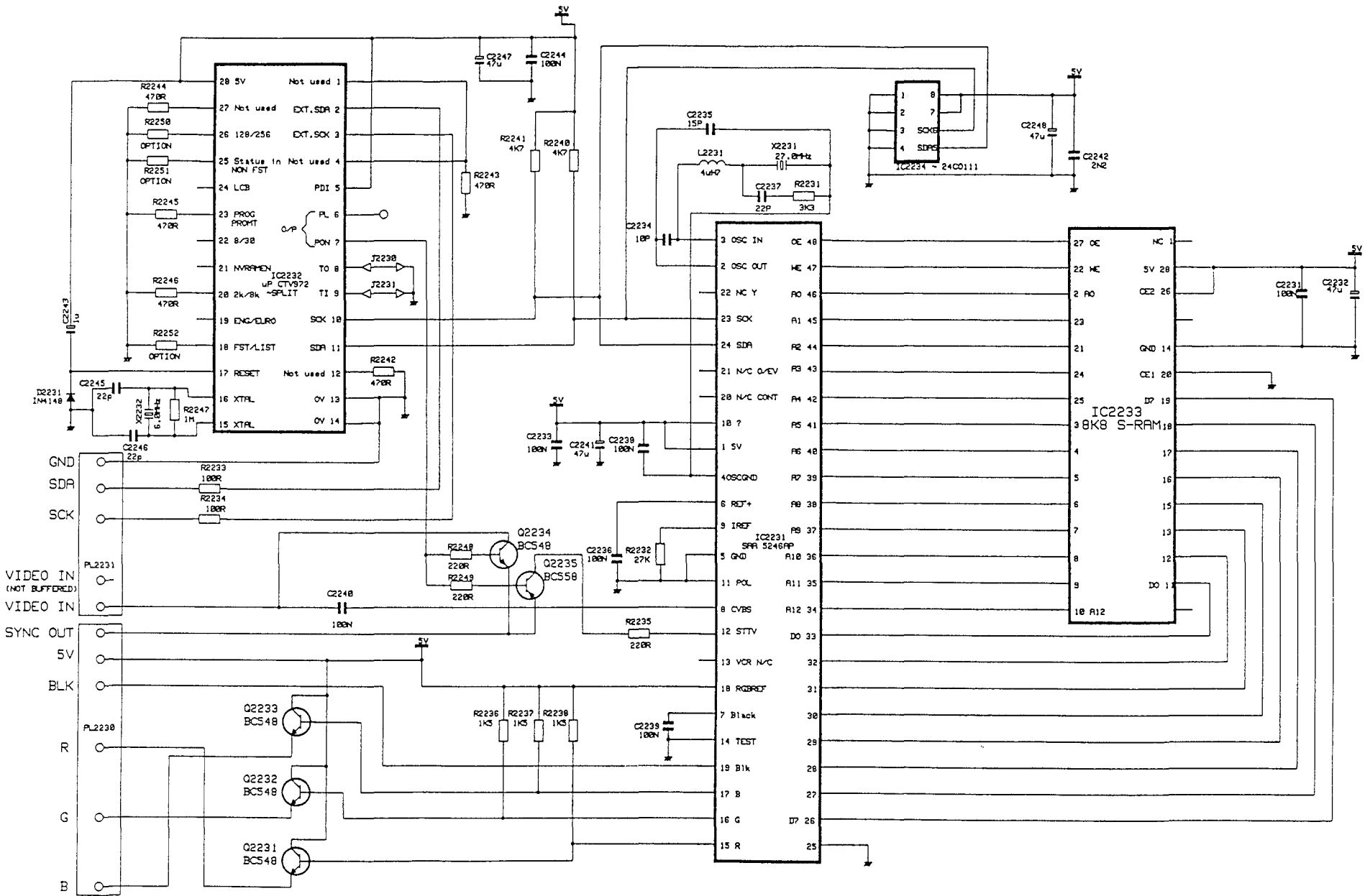
THIS CIRCUIT SUITS PC383.
