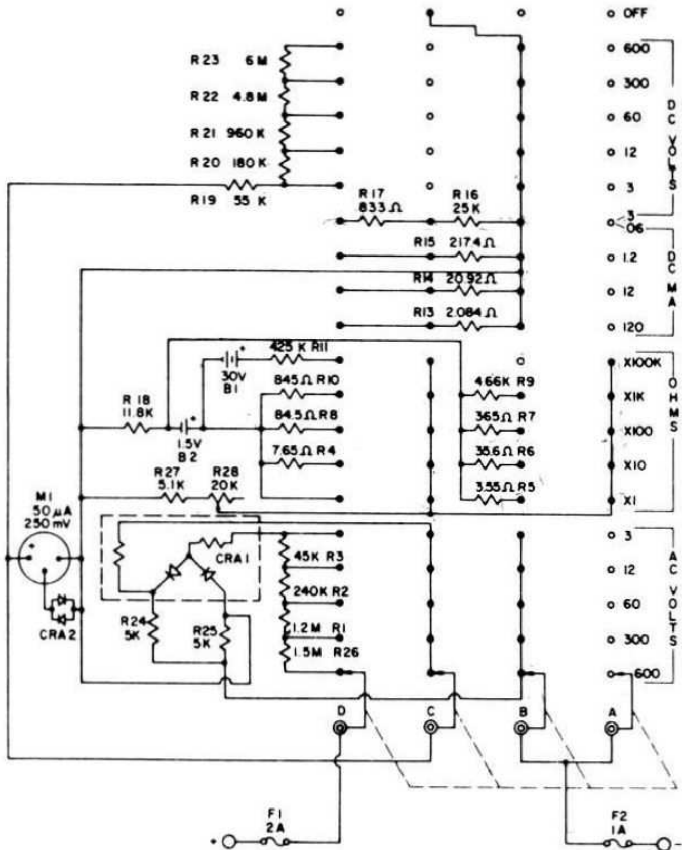
SCHMATIC
