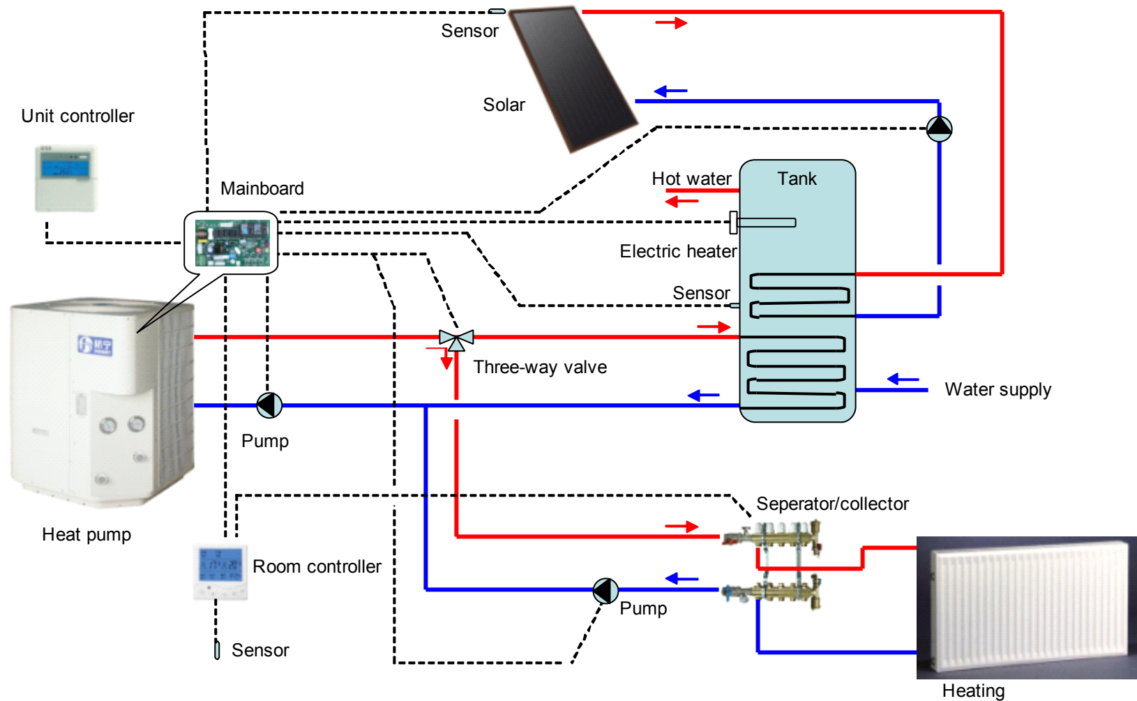
HOT WATER & HEATING SYSTEM DIAGRAM 2
