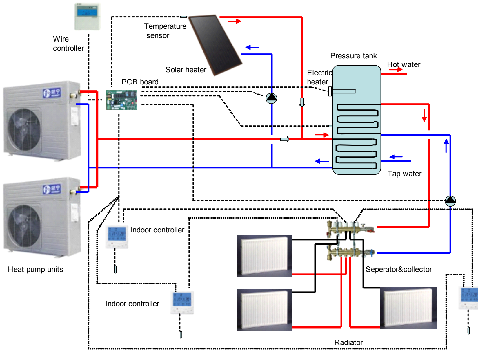
HOT WATER&HEATING DIAGRAM 1
