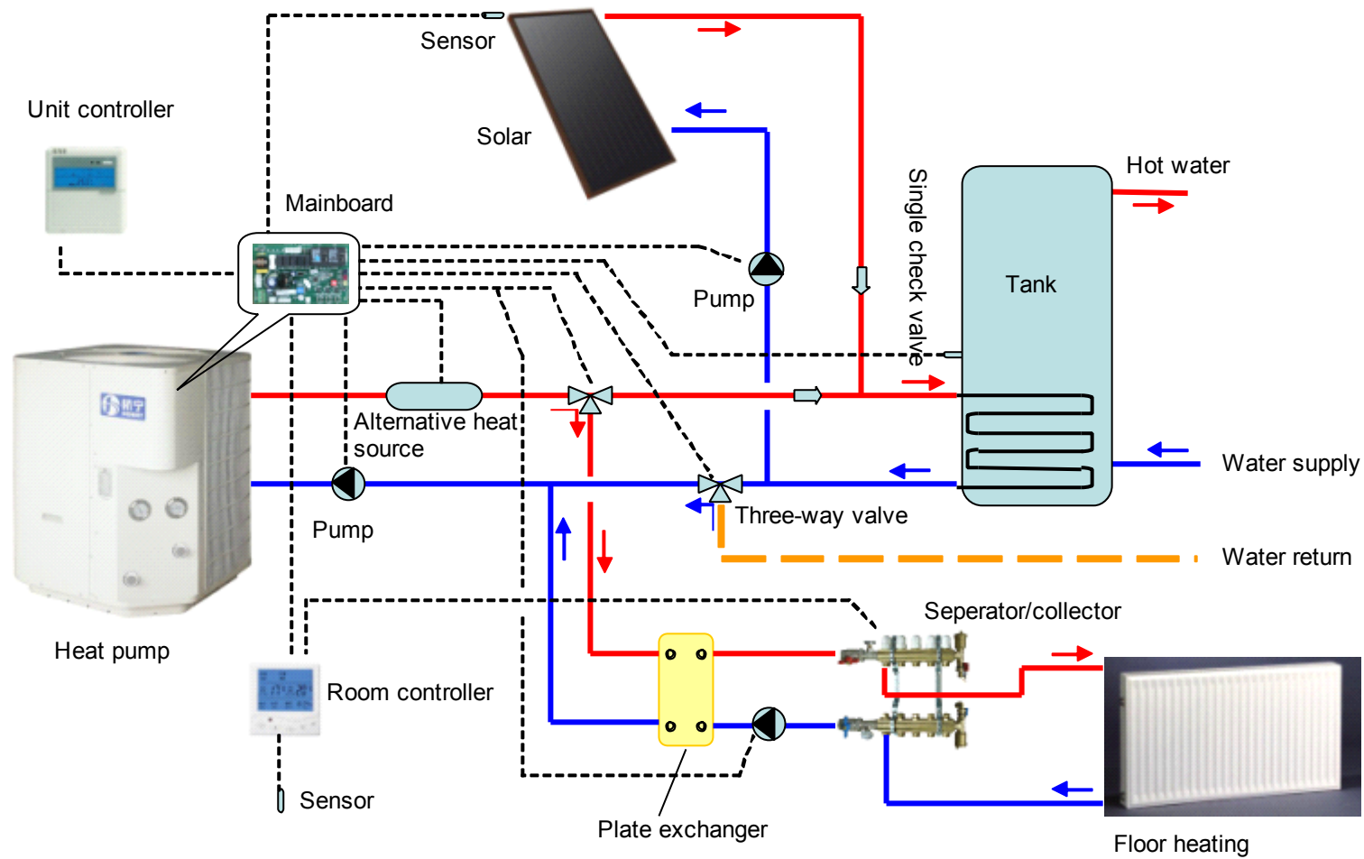
HOT WATER & HEATING SYSTEM DIAGRAM 1
