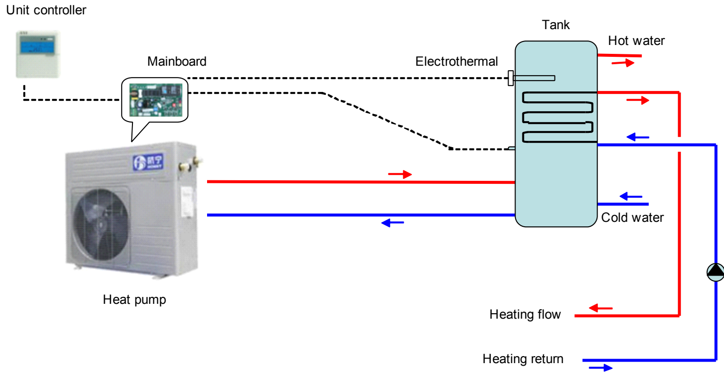
HOT WATER & HEATING SYSTEM DIAGRAM 1
