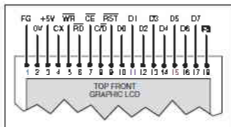
Fig.3. Pinout details from the l.c.d. to the circuit board
