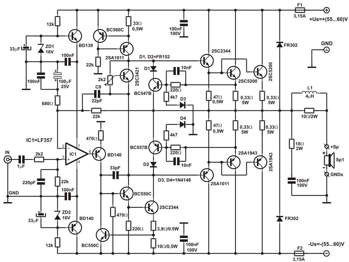
Hi-Fi AUDIO AMPLIFIER "SONATA-100"
