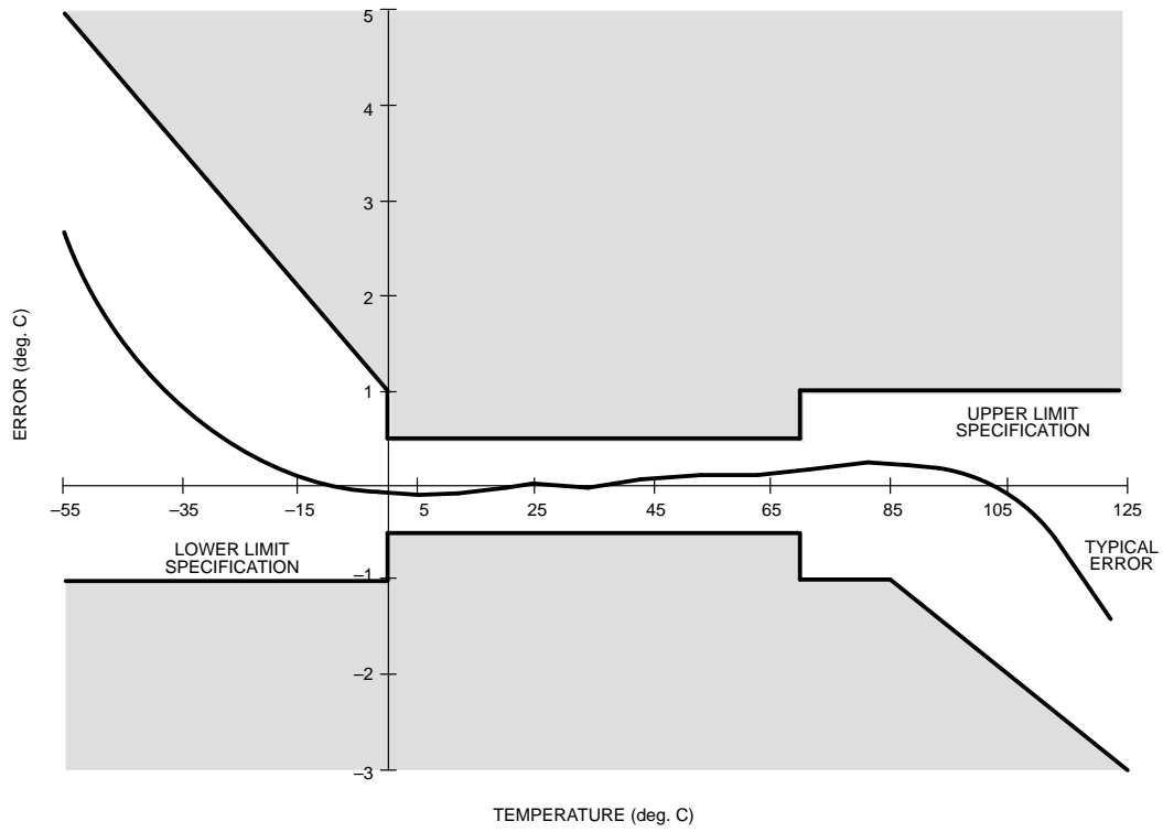
DS1820 DIGITAL TERMOMETER AND THERMOSTAT TEMPERATURE READING ERROR
