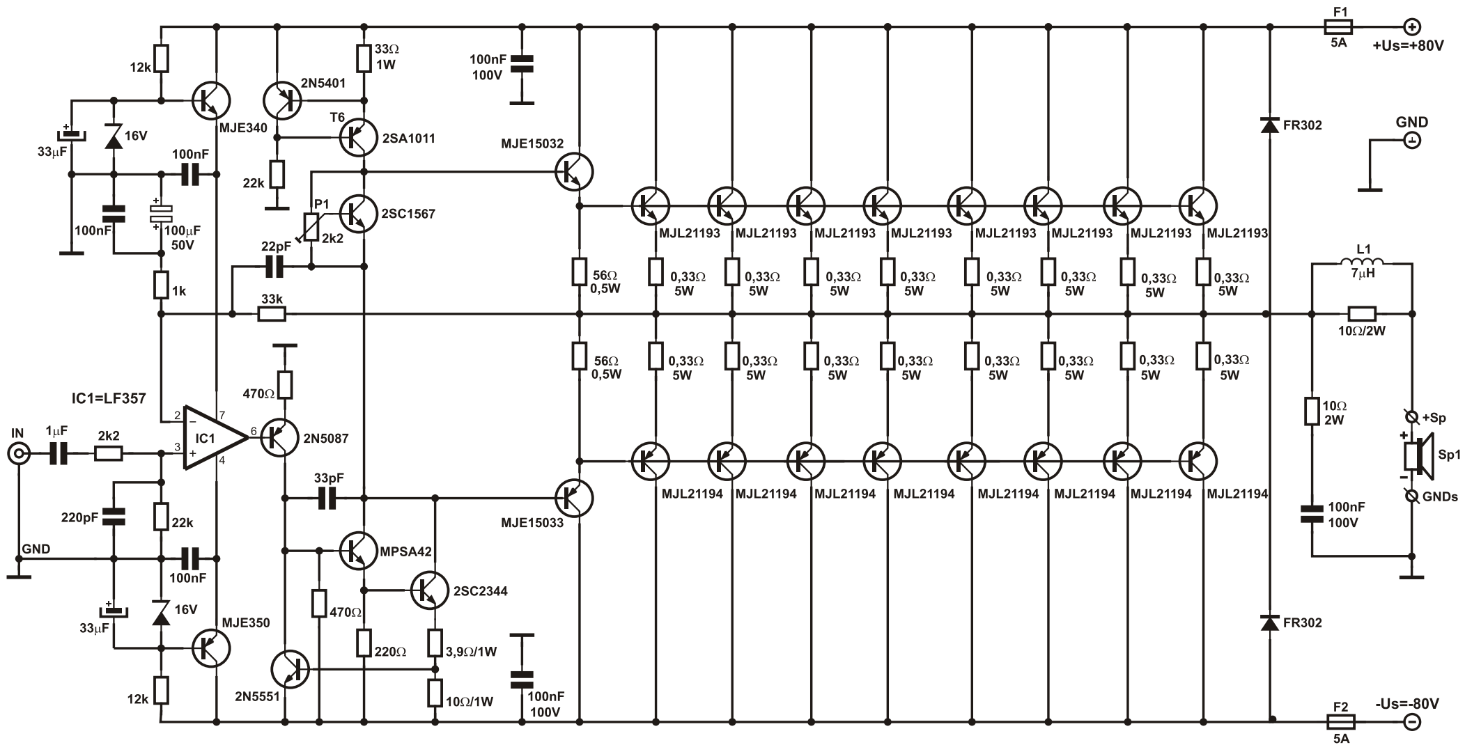
HI-FI AUDIO AMPLIFIER "GLADIATOR-600W"
