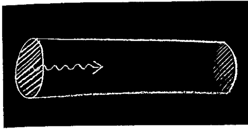
A light pulse is emitted at one end of a hollow cylinder and absorbed at the other end in a thought experiment described 9 by Einstein in 1906. Taking E/c as the momentum of the photon and requiring that the center of mass of the system not move leads to the conclusion that light with energy E transfers mass m = E/c^2 .
