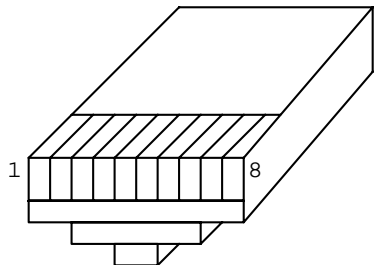
RJ-45 Layout
